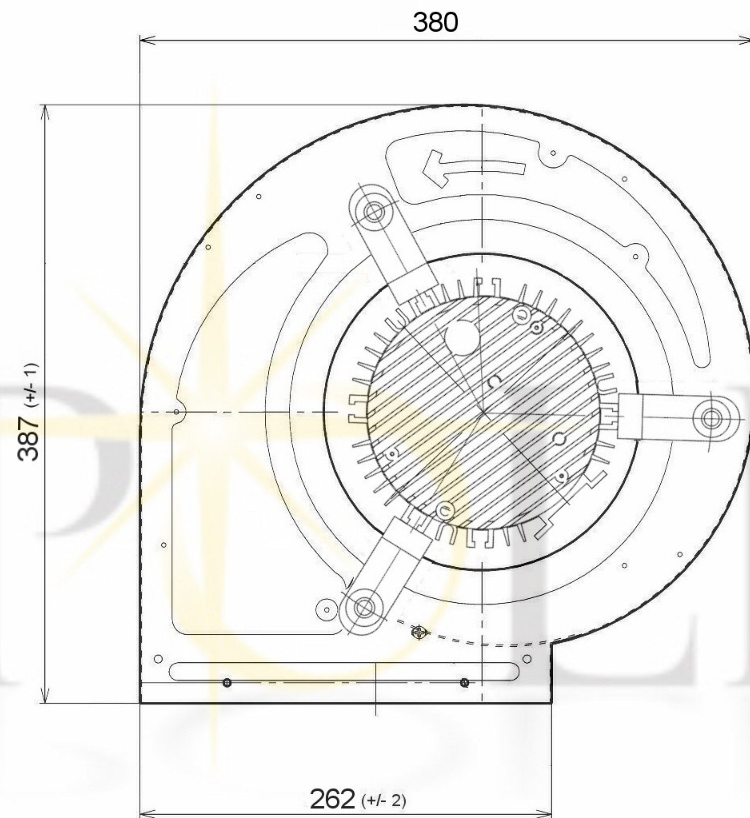
Accessories - DDF9/9 (Mounting Feet)
