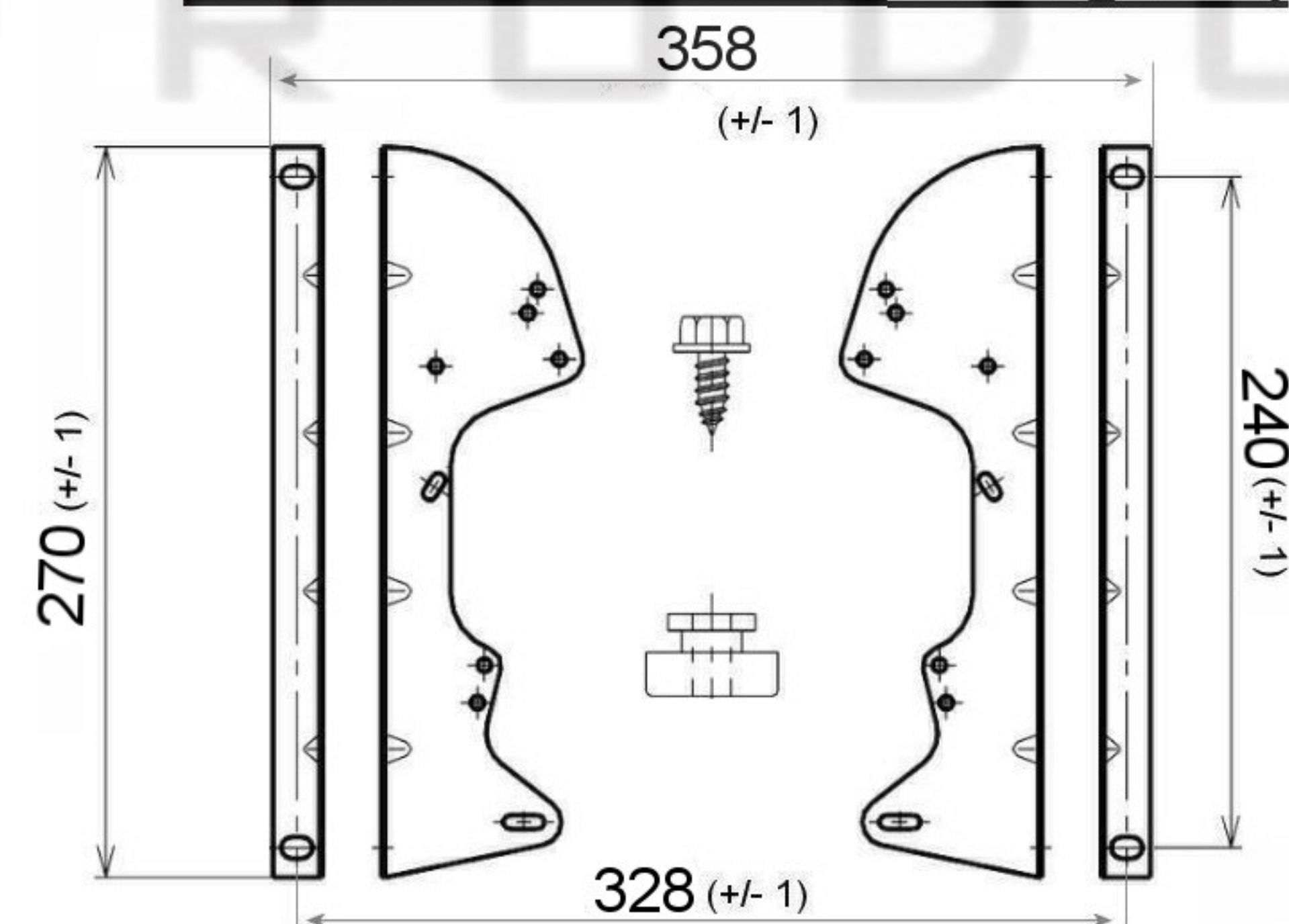
Accessories - DDF9/9 (Mounting Feet)
