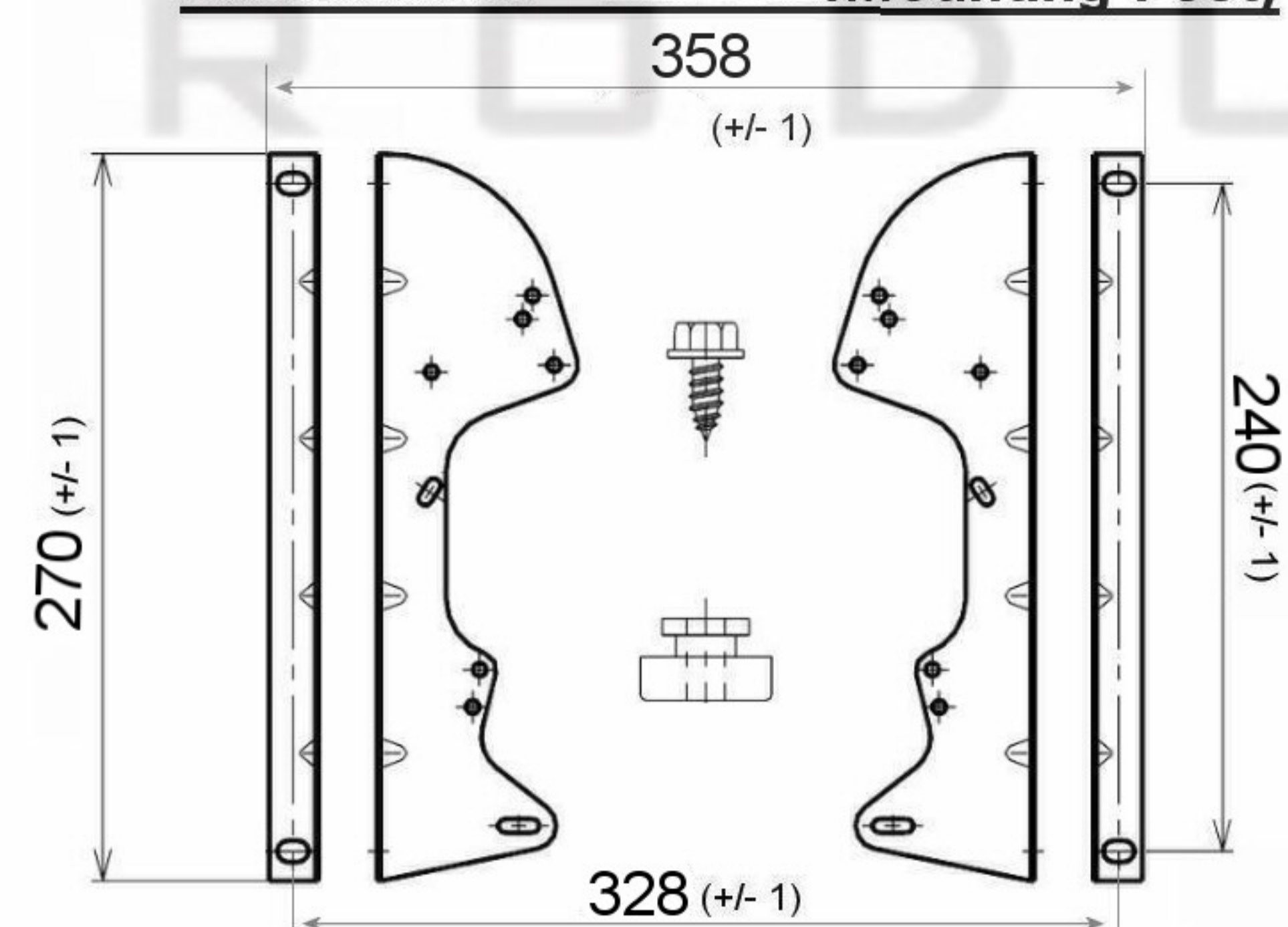
Accessories - DDF9/9 (Mounting Feet)
