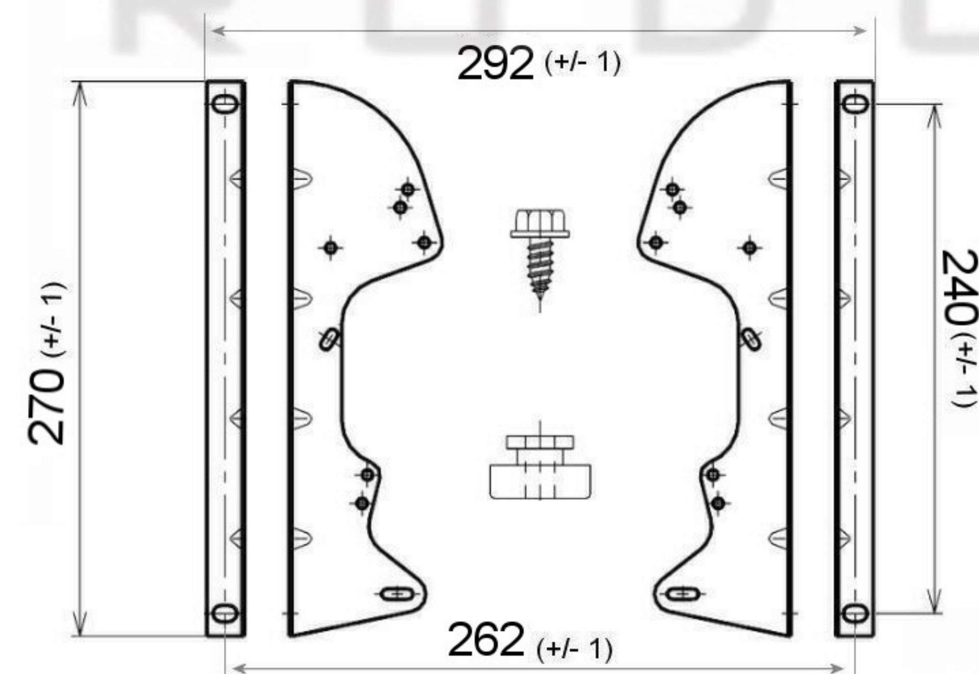
Accessories - DDF9/7 (Mounting Feet)
