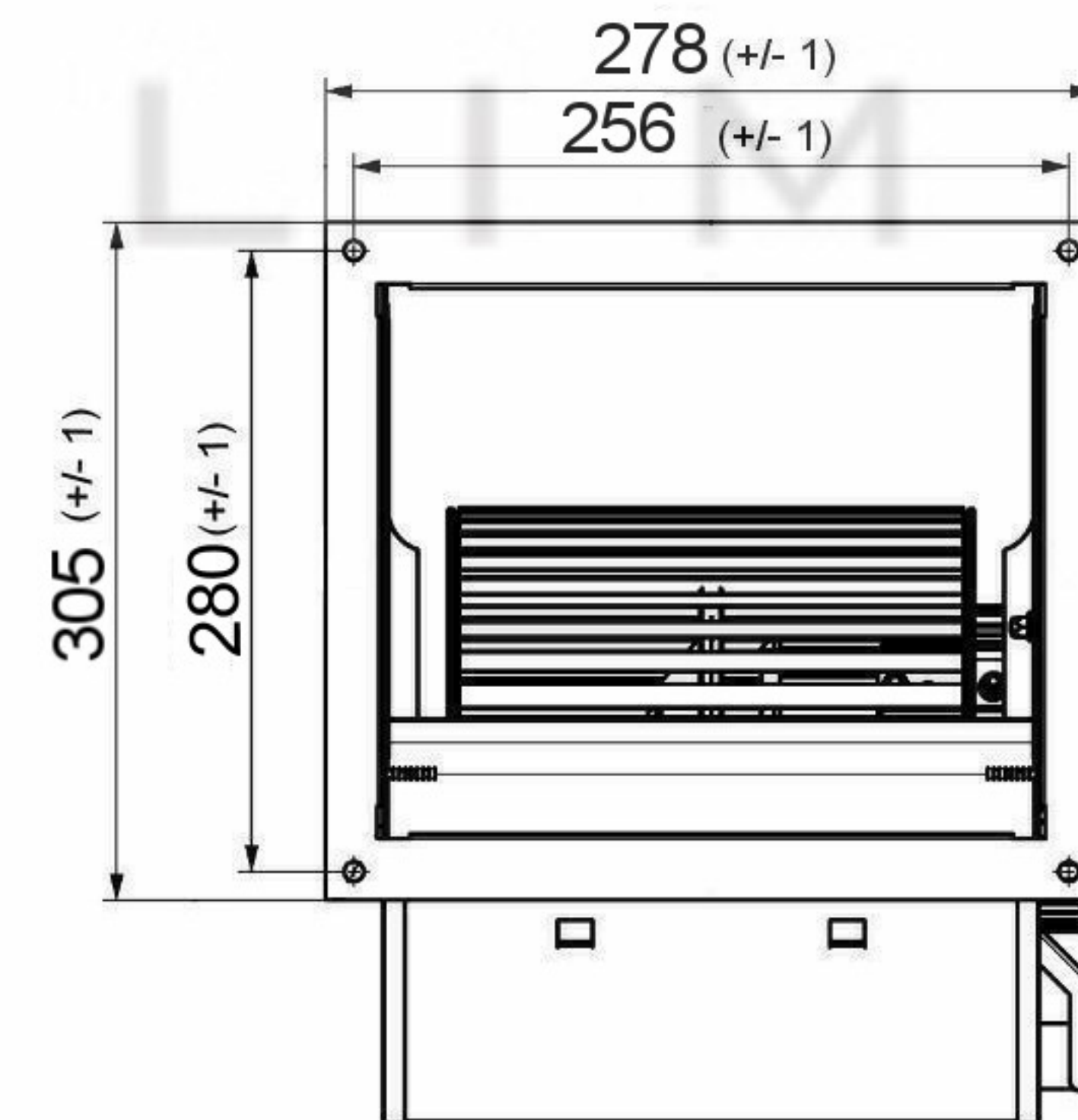
Accessories - DD9F (Flange)
