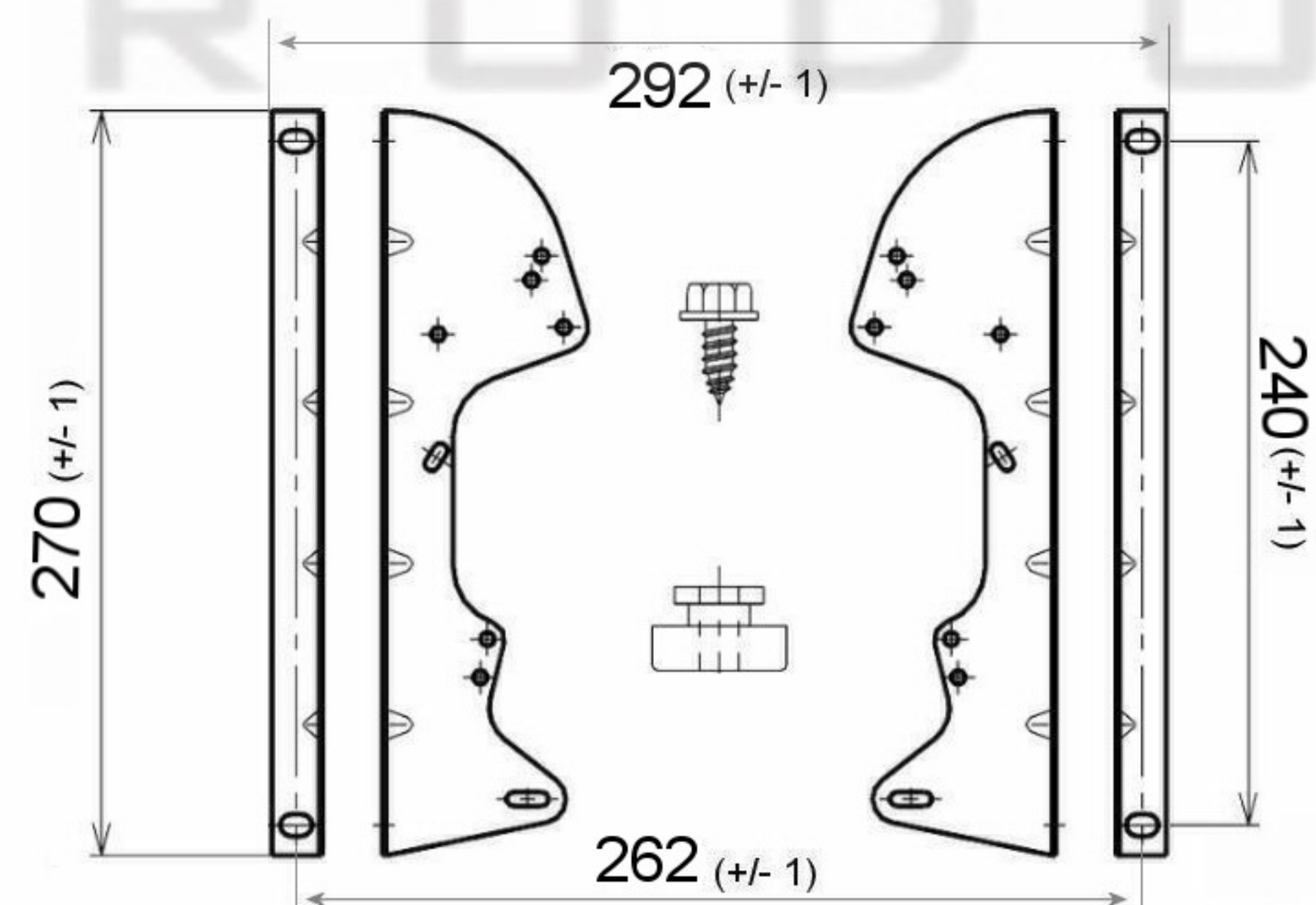
Accessories - DDF9/7 (Mounting Feet)
