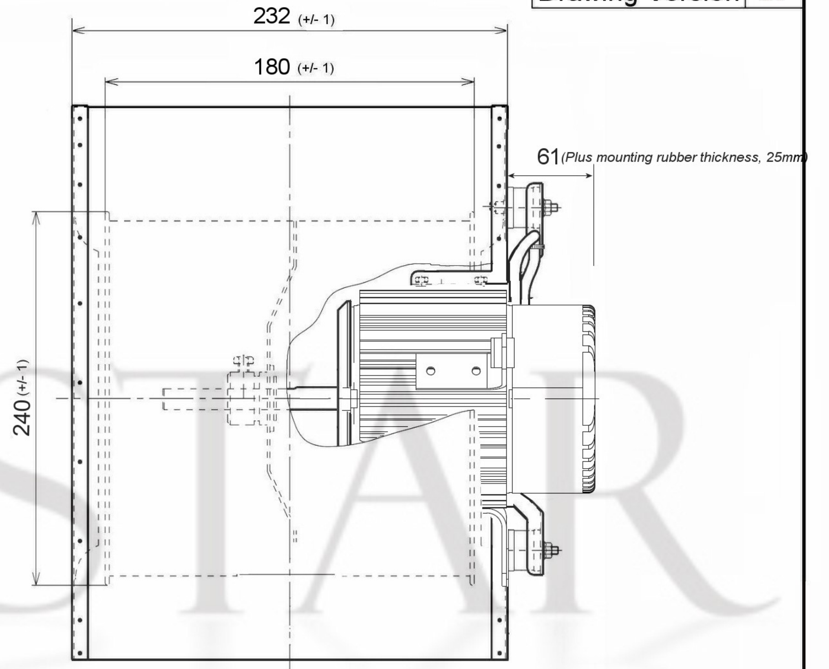
Accessories - DD9F (Flange)
