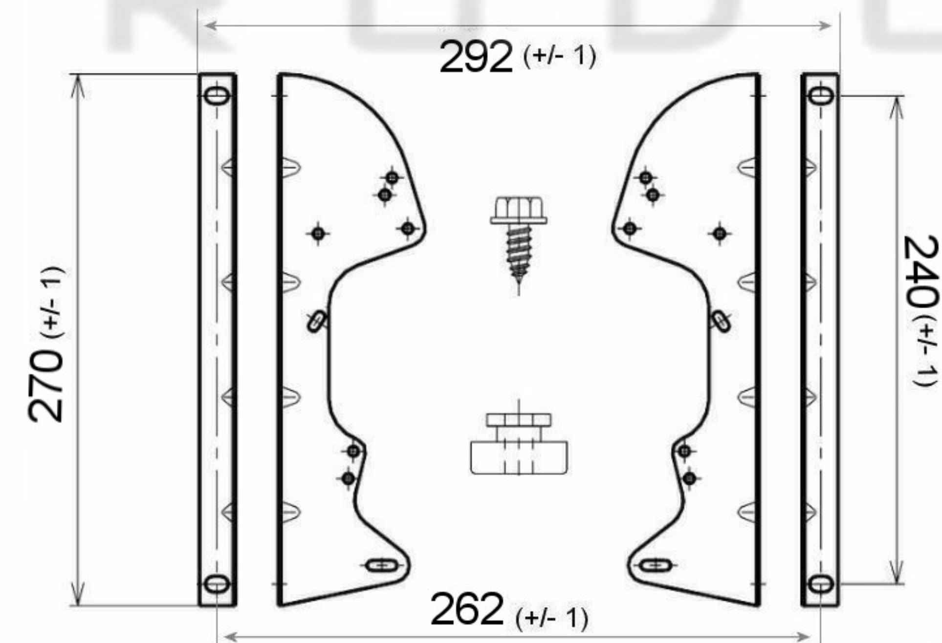
Accessories - DDF9/7 (Mounting Feet)
