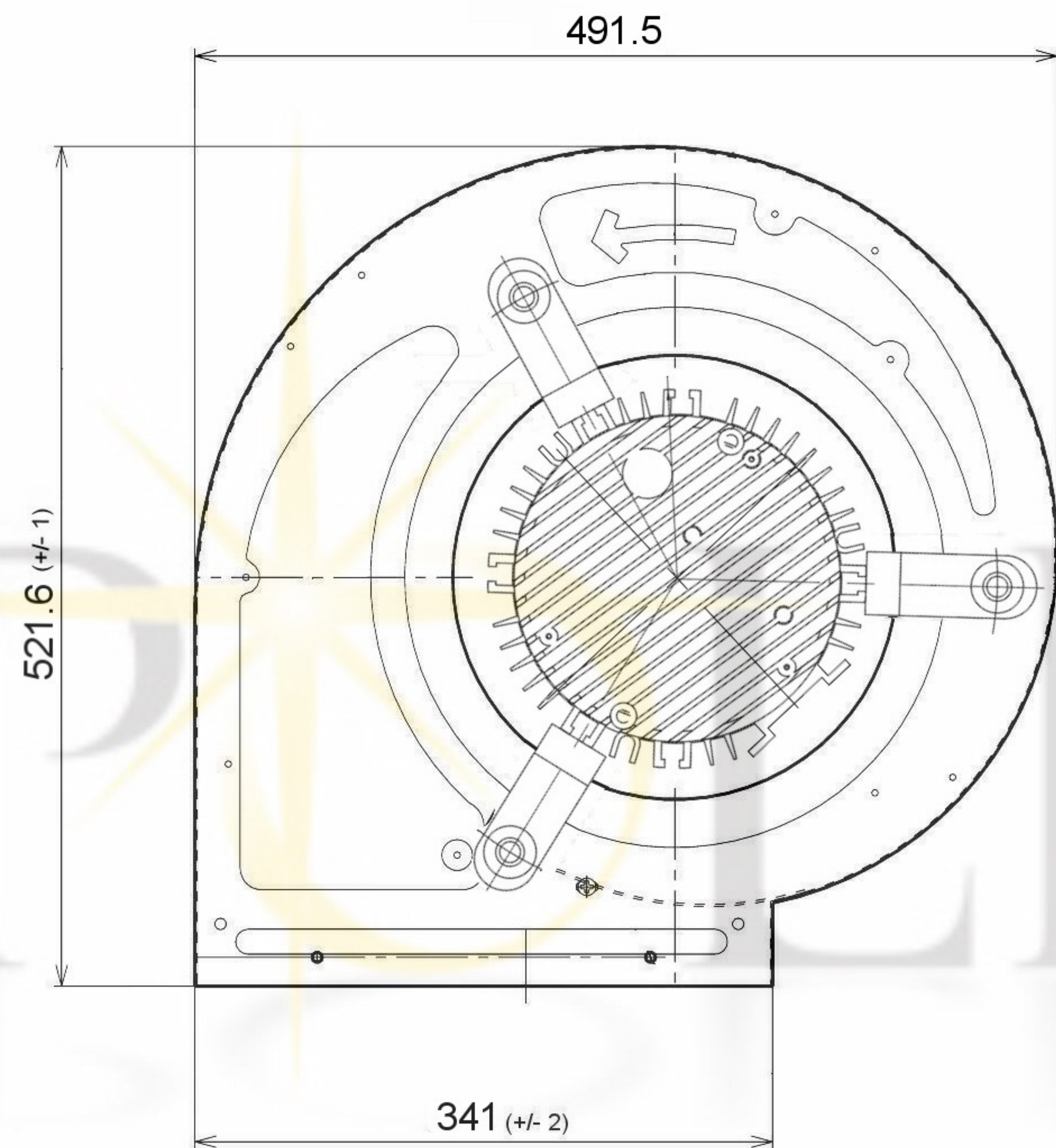
Accessories - DD12F (Mounting Feet)
