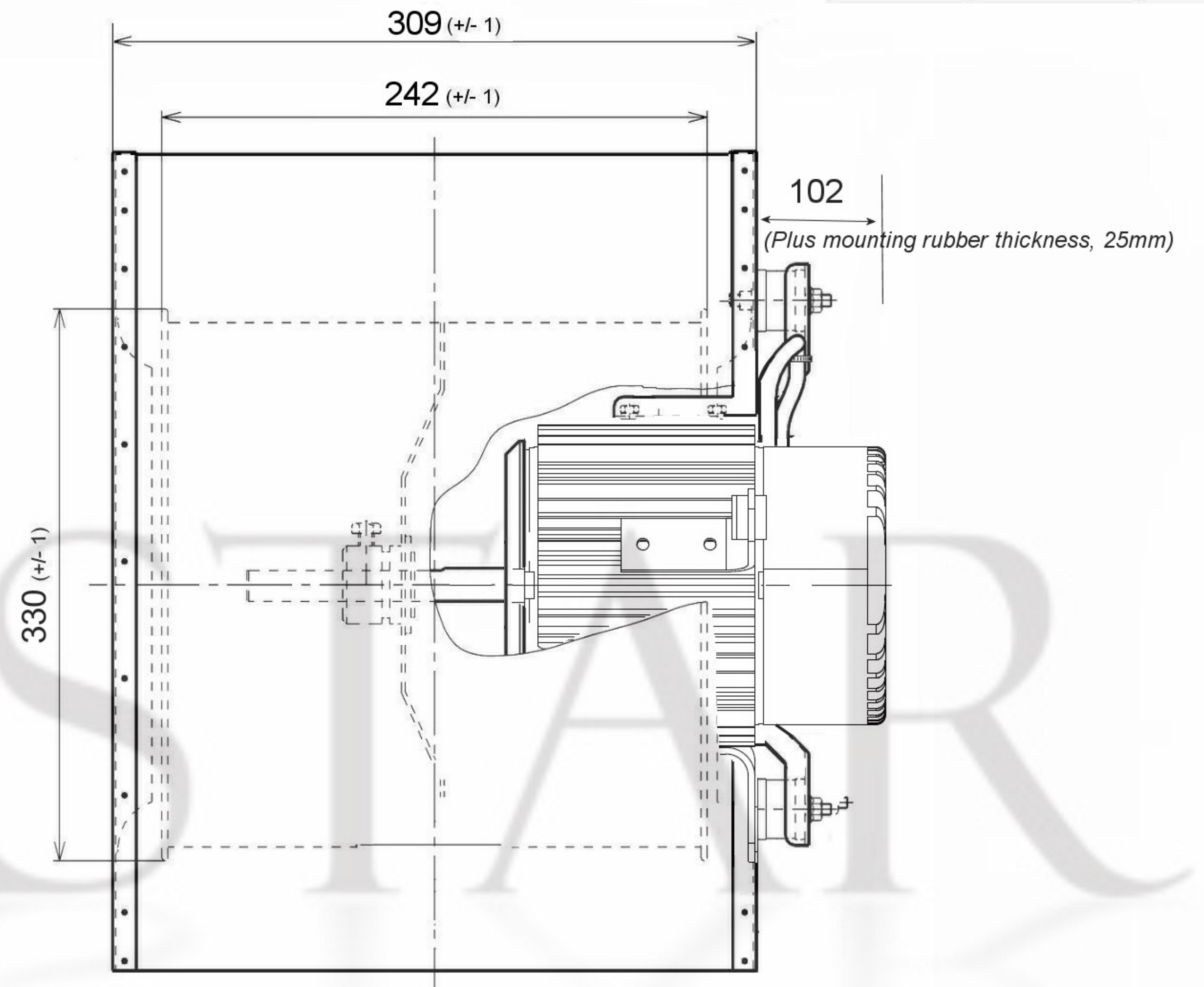
Accessories - DDF12/9 (Flange)
