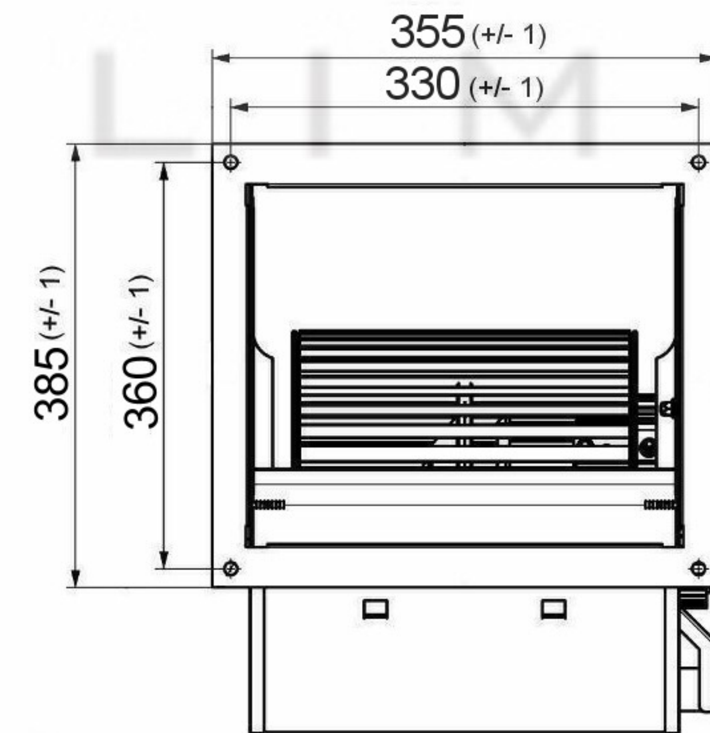
Accessories - DDF12/9 (Flange)
