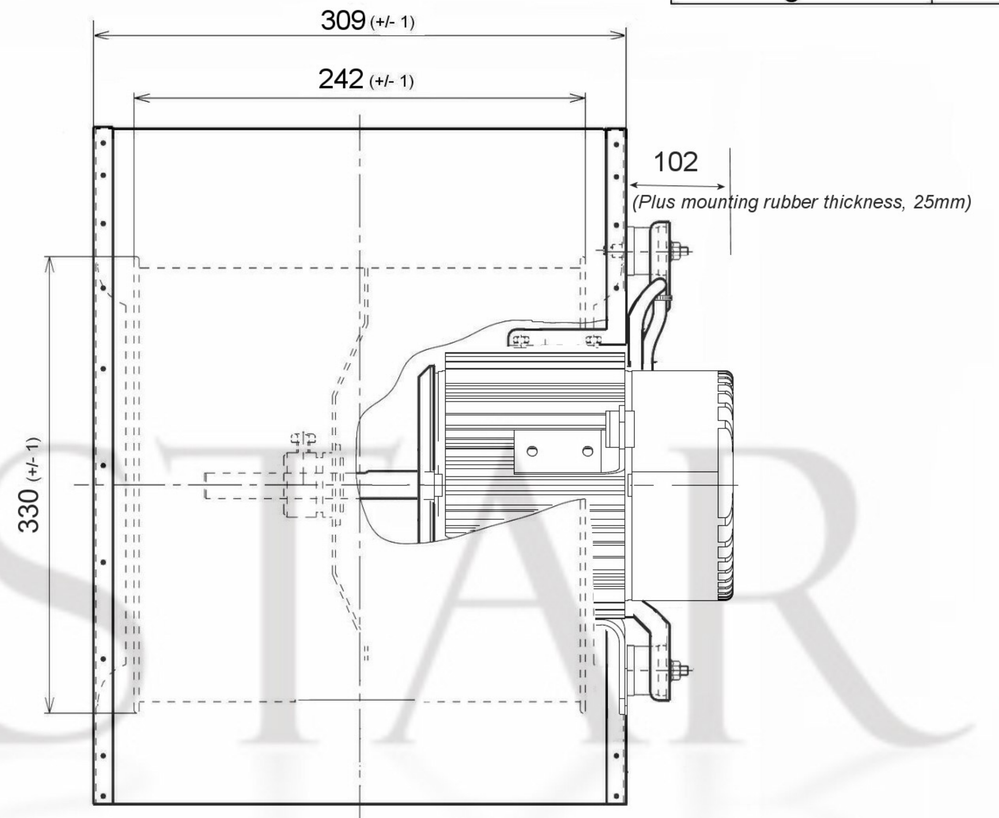
Accessories - DDF12/9 (Flange)
