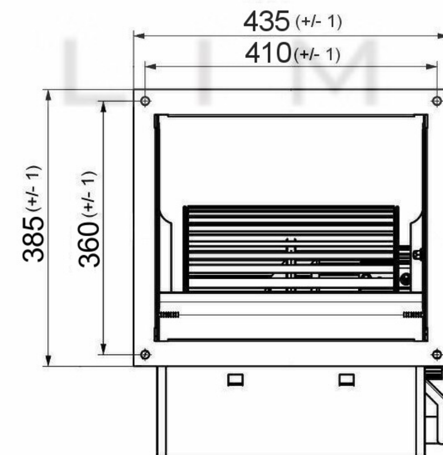
Accessories - DDF12/12 (Flange)
