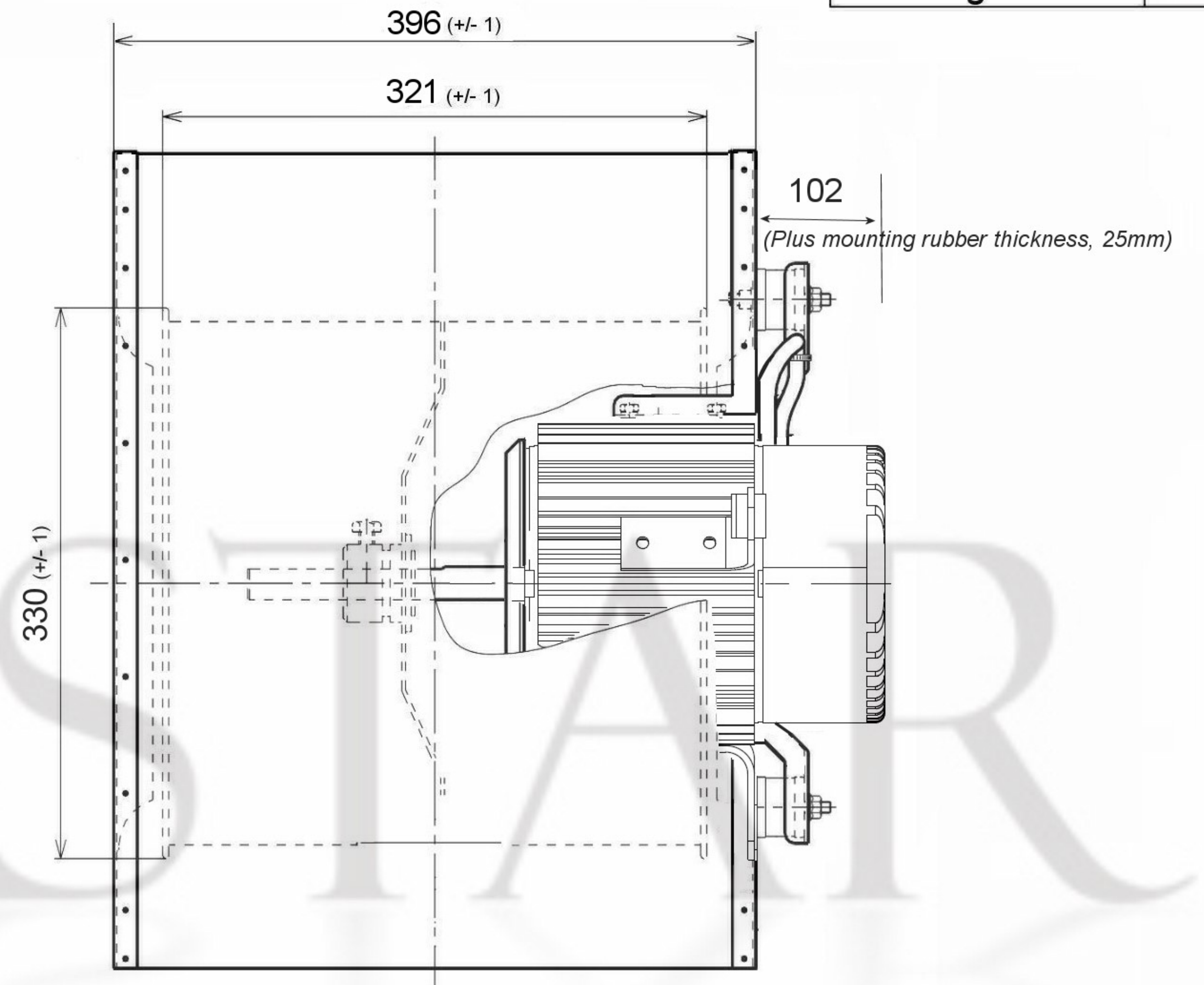
Accessories - DDF12/12 (Flange)
