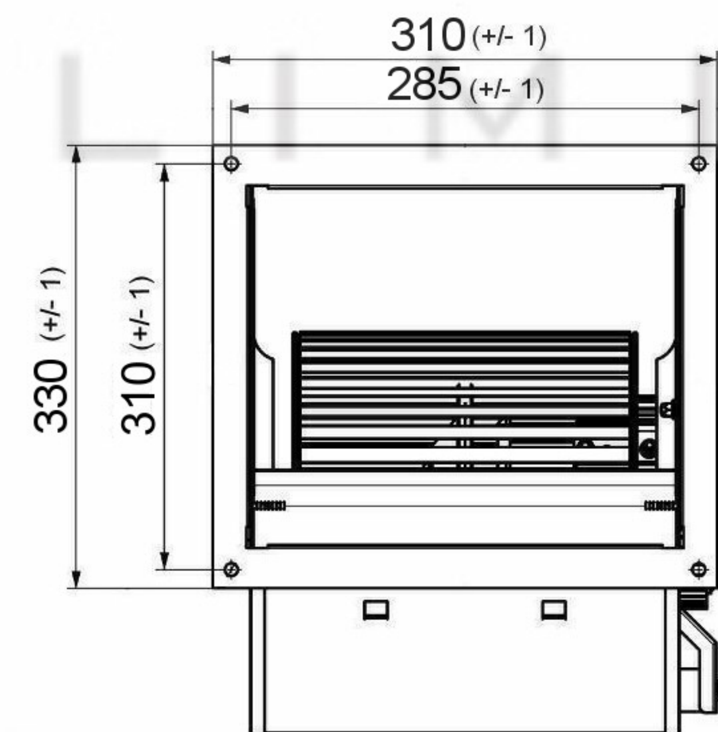
Accessories - DDF10/8 (Flange)
