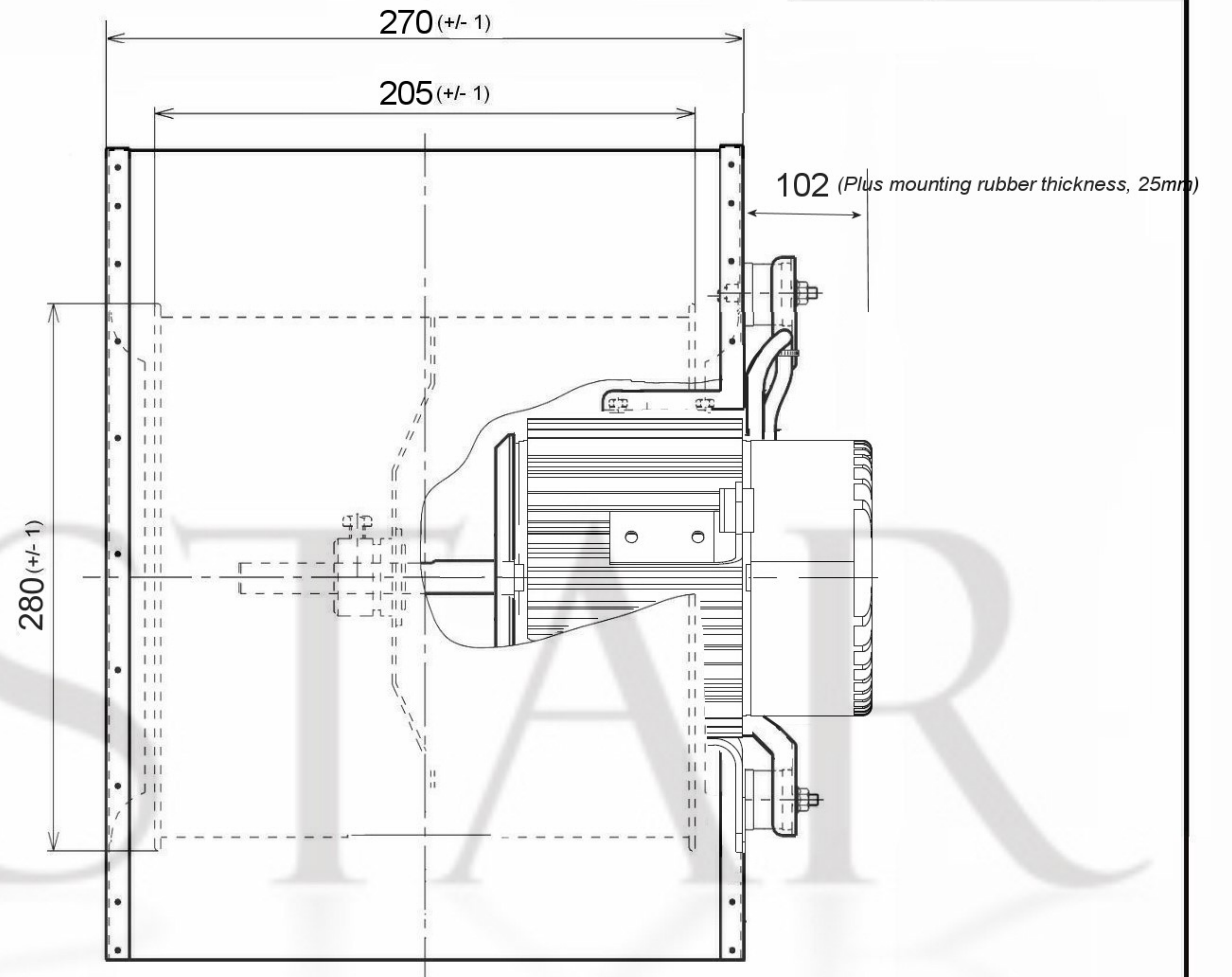
Accessories - DDF10/8 (Flange)
