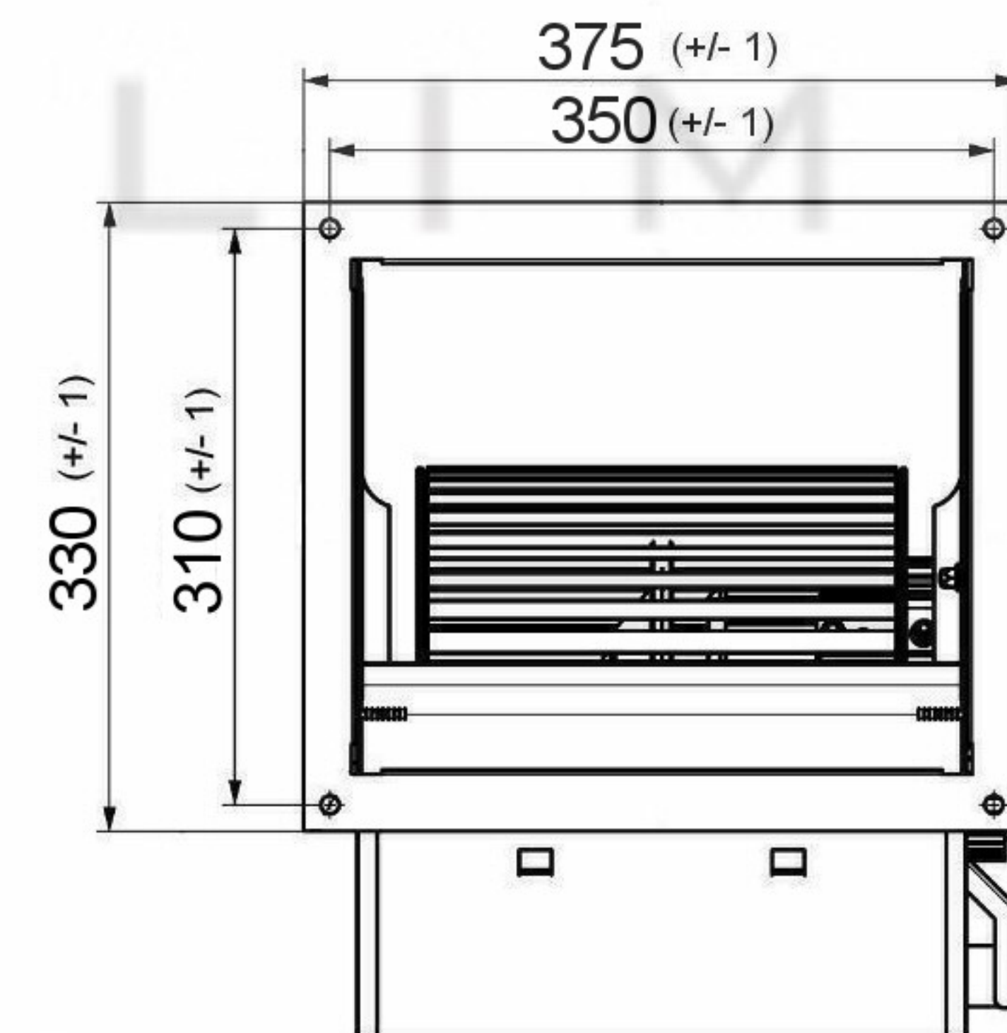
Accessories -DDF10/10(Flange)
