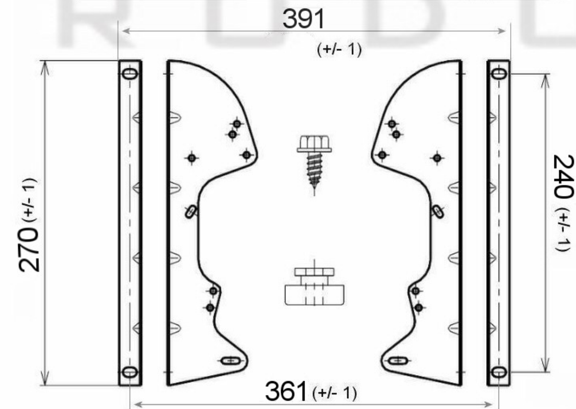
Accessories -DD10F (Mounting Feet)
