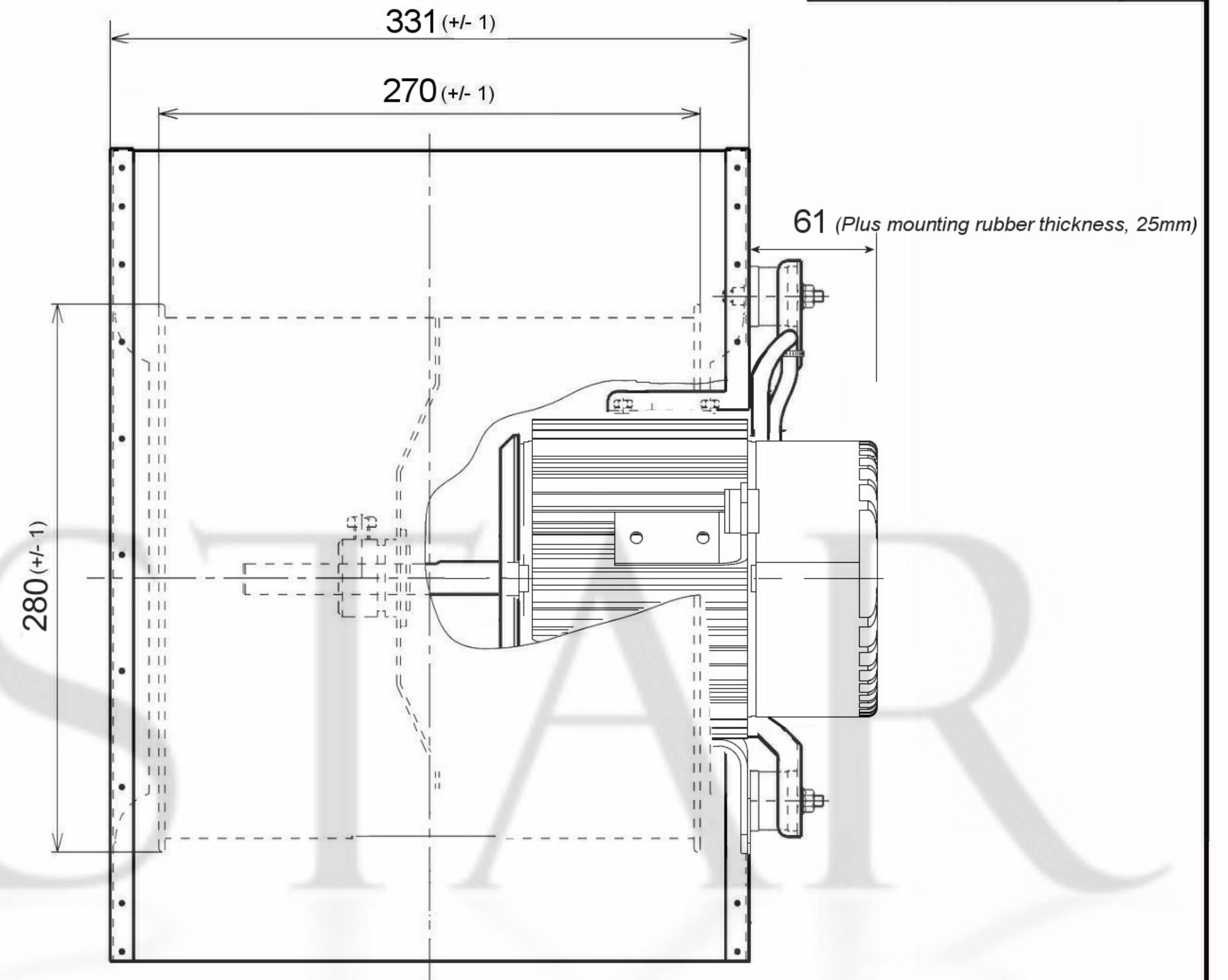
Accessories -DDF10/10(Flange)
