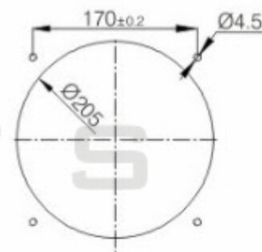
mounting dimension
