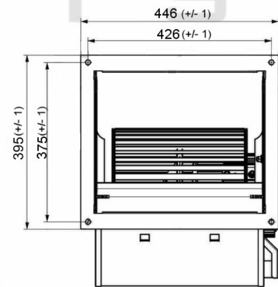
Accessories: DDF12/12 (Mounting Flange)
