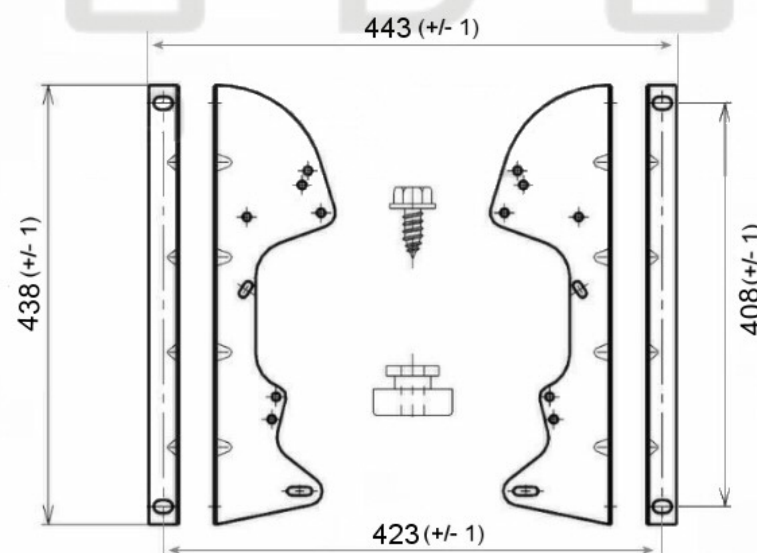
Accessories: DD12F (Mounting Feet)
