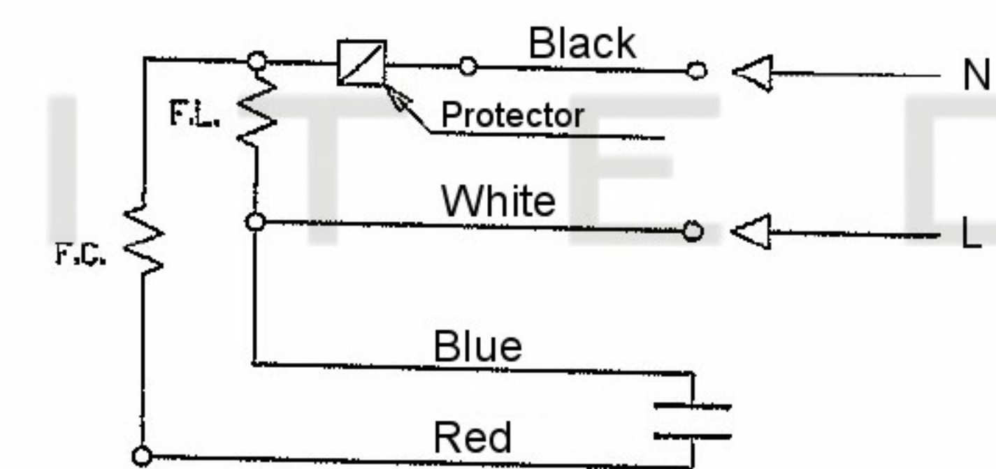
Wiring Details
