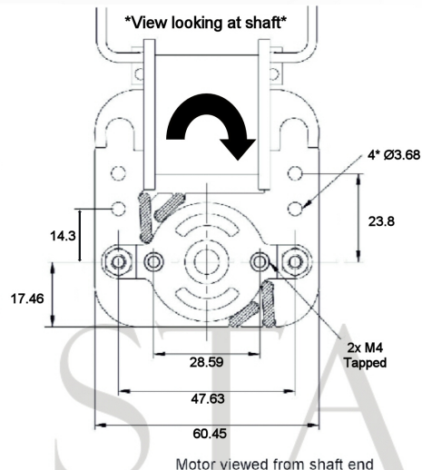
Motor viewed from shaft end
