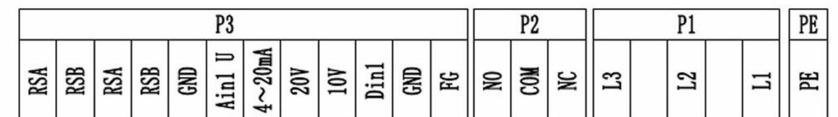
Wiring diagram
