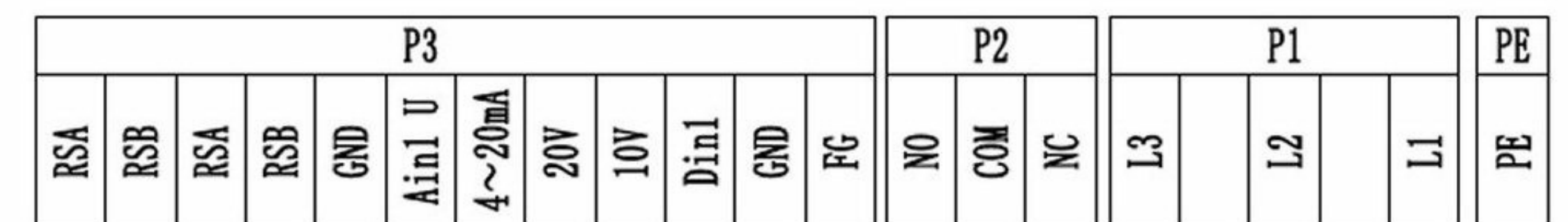
Wiring diagram
