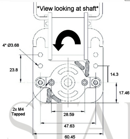
Motor viewed from shaft end
