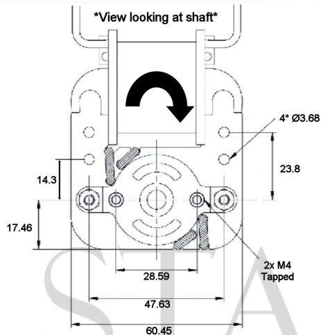
Motor viewed from shaft end
