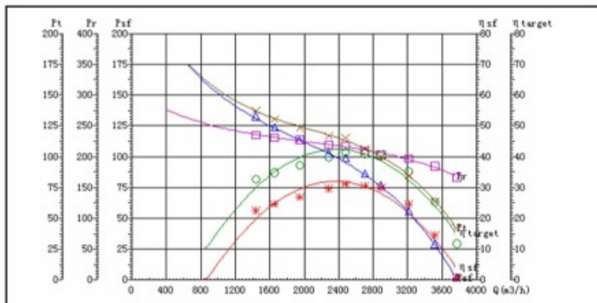
Performance Curve
