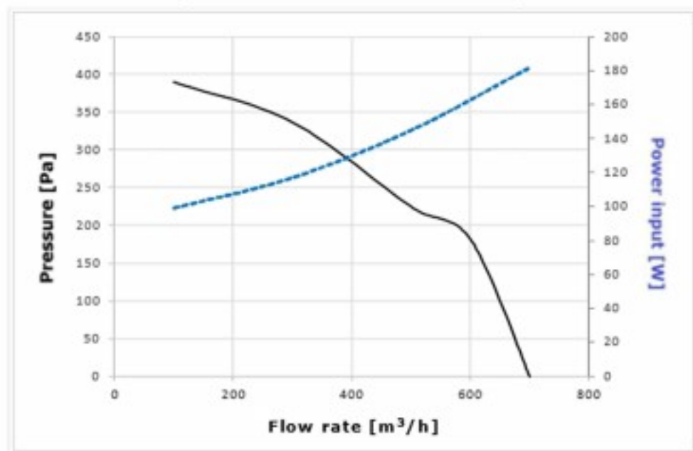
Air flow performance at 230V 50Hz
